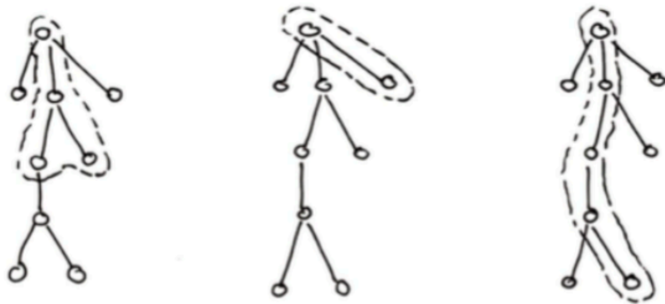
TOP-DOWN SUBTREE
